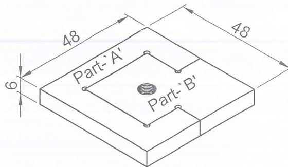
Assemble Part-A & Part-B
